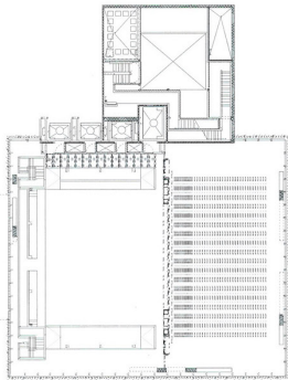
Planta segunda / Second floor plan
