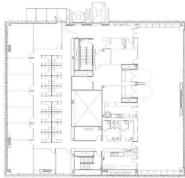
Planta séptima / Seventh floor plan
