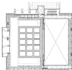
Planta tercera / Third floor plan
